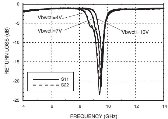
Return Loss vs. Vbwctl, Vfctl = 7V
